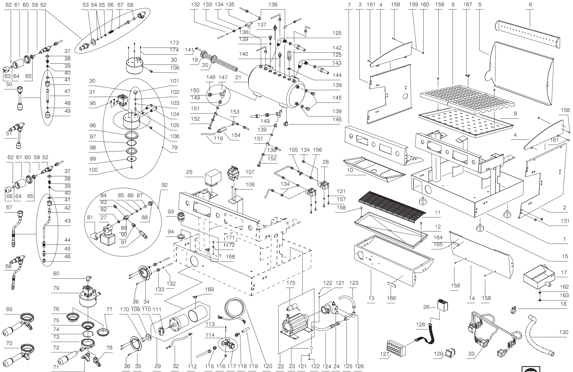
Exploded view CAPRI update 09-05
