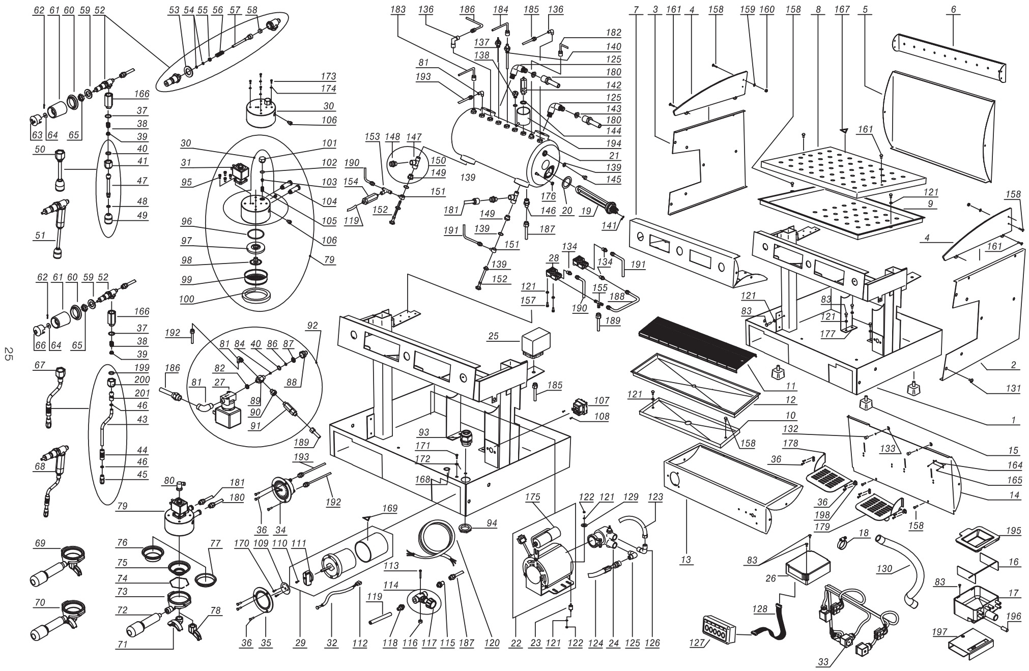
Mod. AMALFI DLX 2GR SED EXPLODED VIEW Update 01-10
