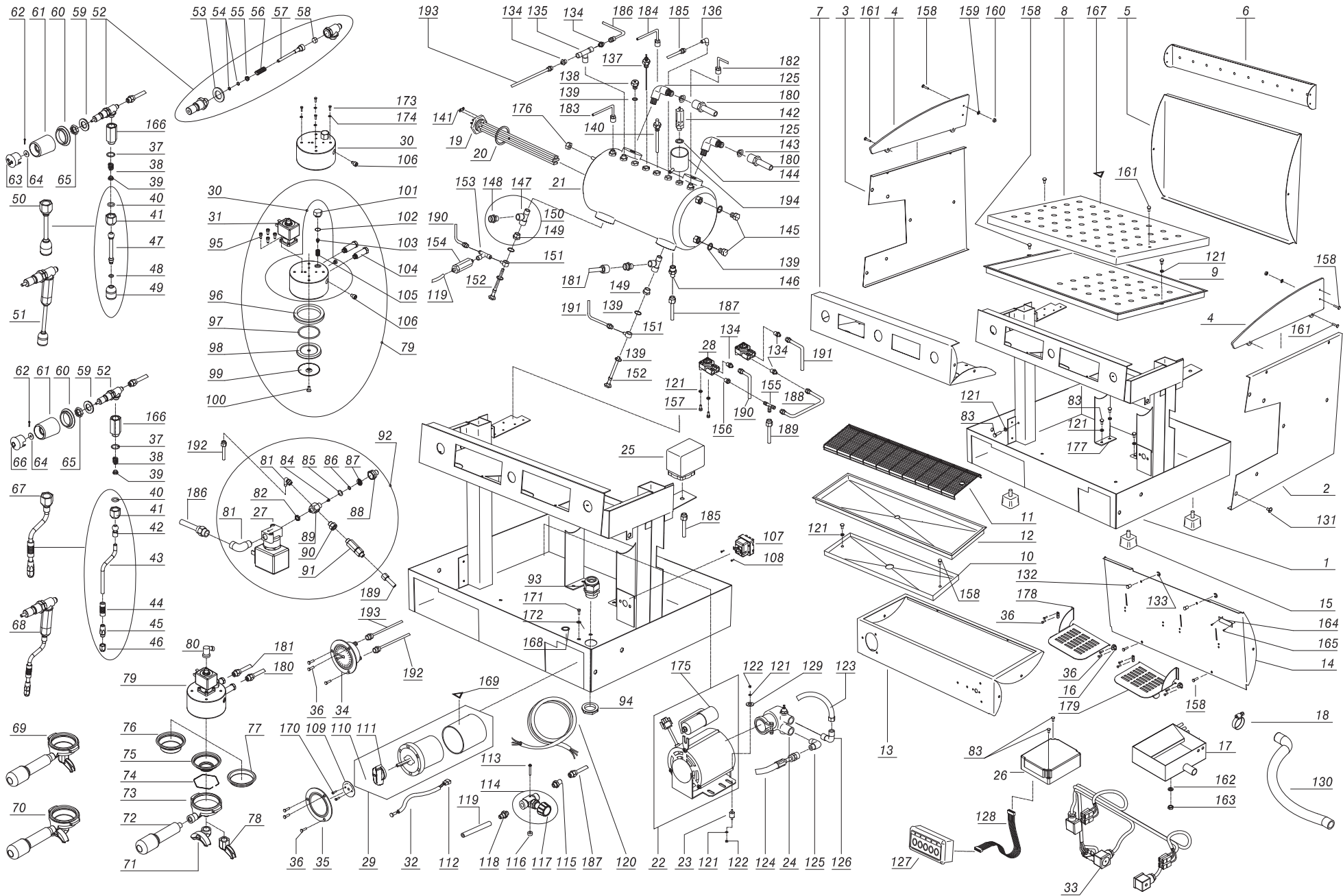
Mod. AMALFI 2GR SED EXPLODED VIEW Update 09-06
